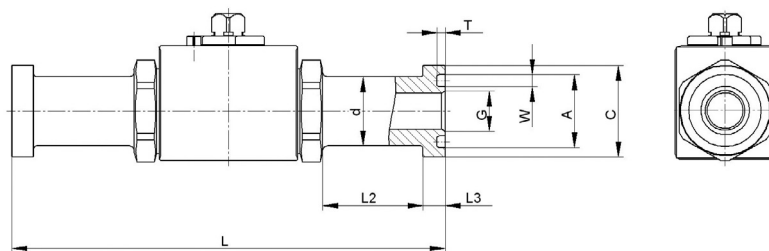
BKH SAE split 3000psi (ISO 6162-1)
