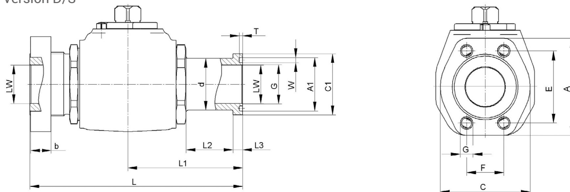
SKH SAE 3000psi (ISO 6162-1)
