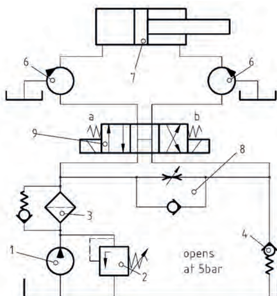
Hydraulic motor pressurised on both sides
