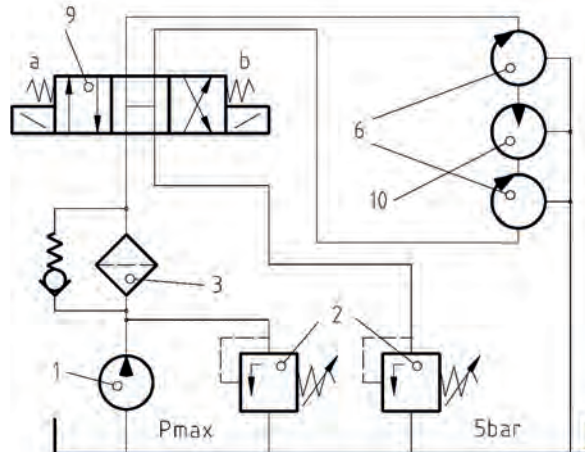
Hydraulic motor pressurised on both sides
