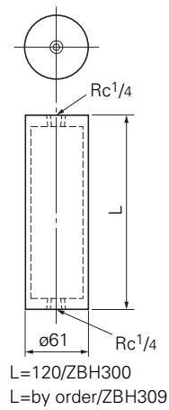
Sealed drain pot (ZBH30)
